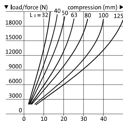
2461.4.063. Ø 63/70 Shore A
