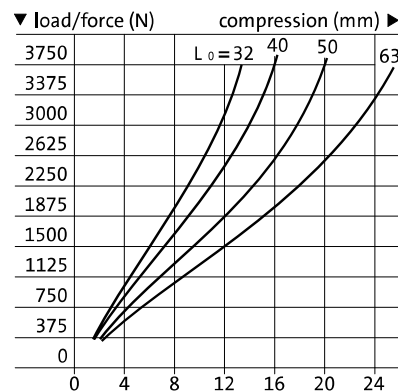
2461.4.032. Ø 32/70 Shore A
